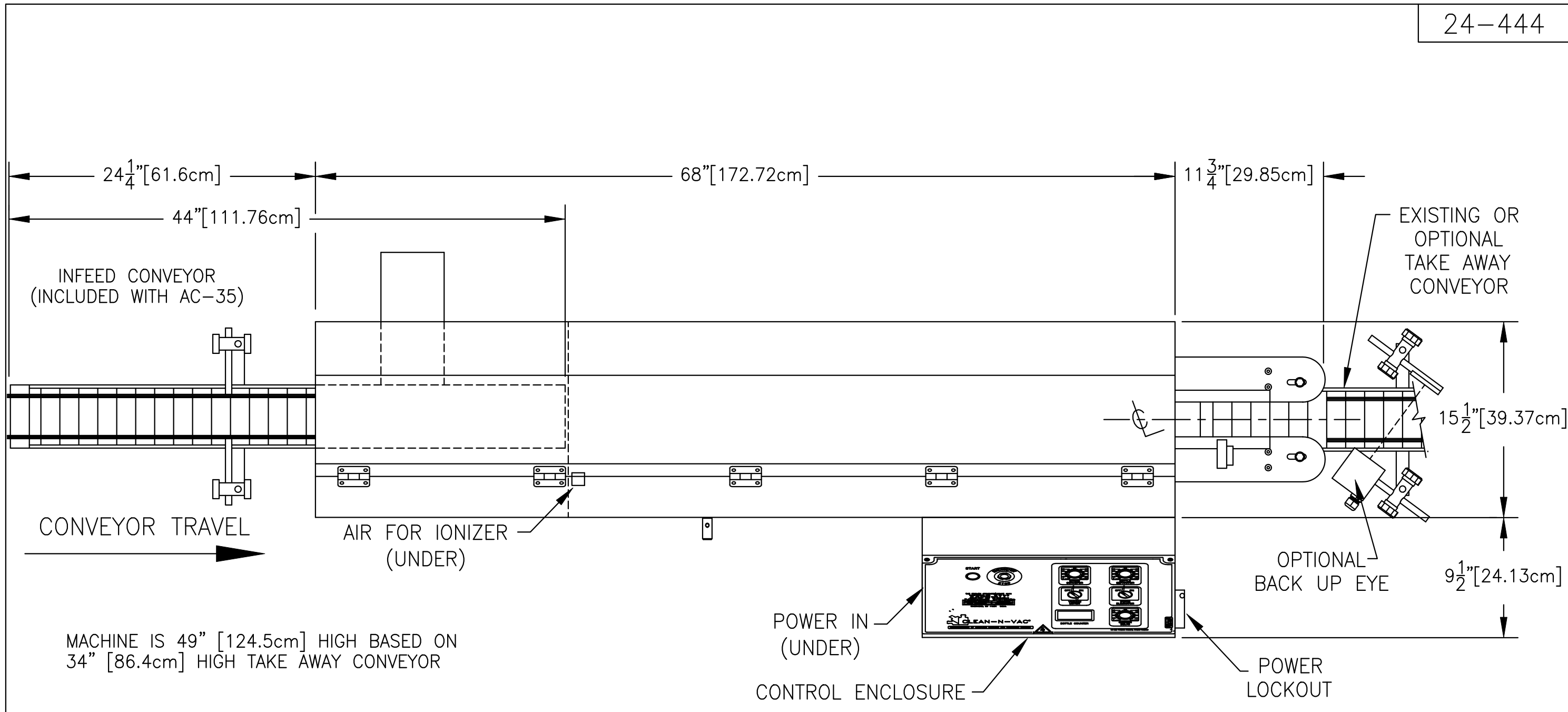
TOP VIEW MODEL AC-35
